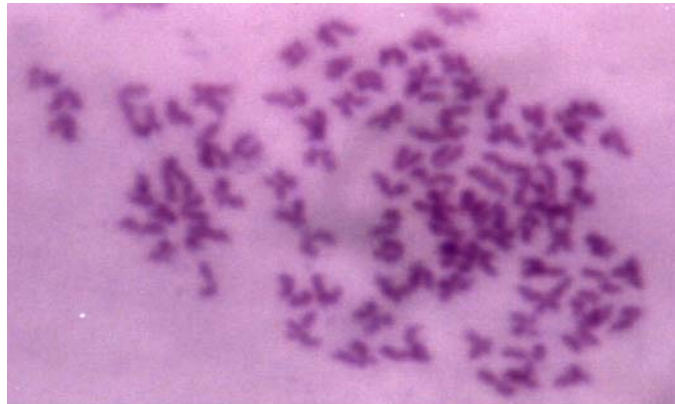
Image 2. Tor khudree chromosome spread
