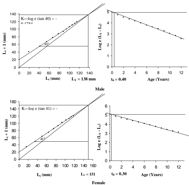
Image 7. Ford-Walford graph of estimating L_{\infty} and t_0 for Salmostoma untrahi for the data obtained by scatter diagram during 2000-01
