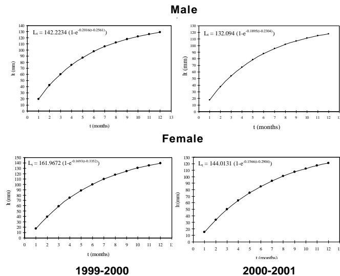
Image 8. Von-Bertalanffy growth curve for Salmostoma untrahi
