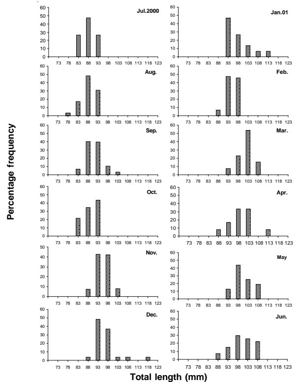
Image 4. Size frequency distribution of female Salmostoma untrahi during July 2000 to June 2001
