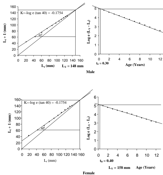
Image 6. Ford-Walford graph of estimating L_{\infty} and t_0 for Salmostoma untrahi for the data obtained by scatter diagram during 1999-2000
