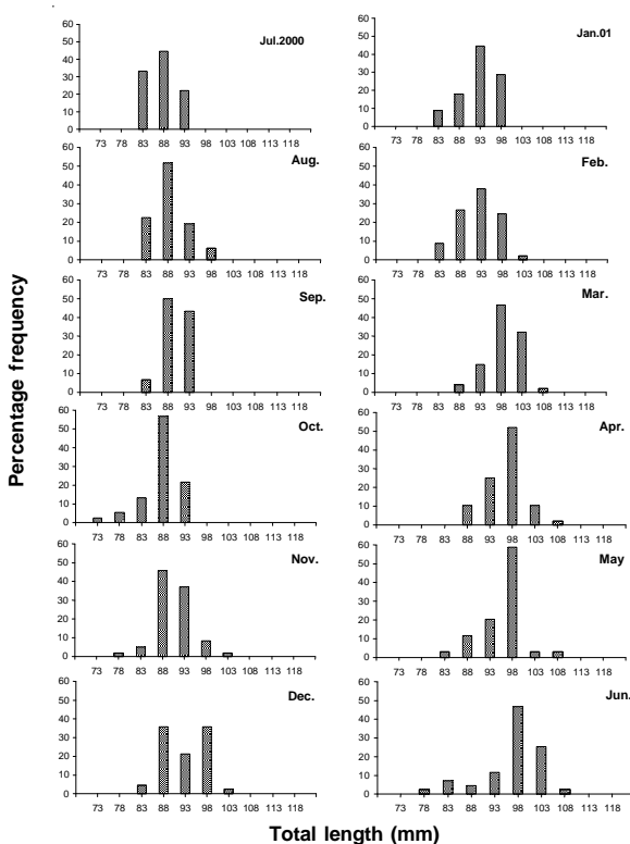
Image 3. Size frequency distribution of male Salmostoma untrahi during July 2000 to June 2001
