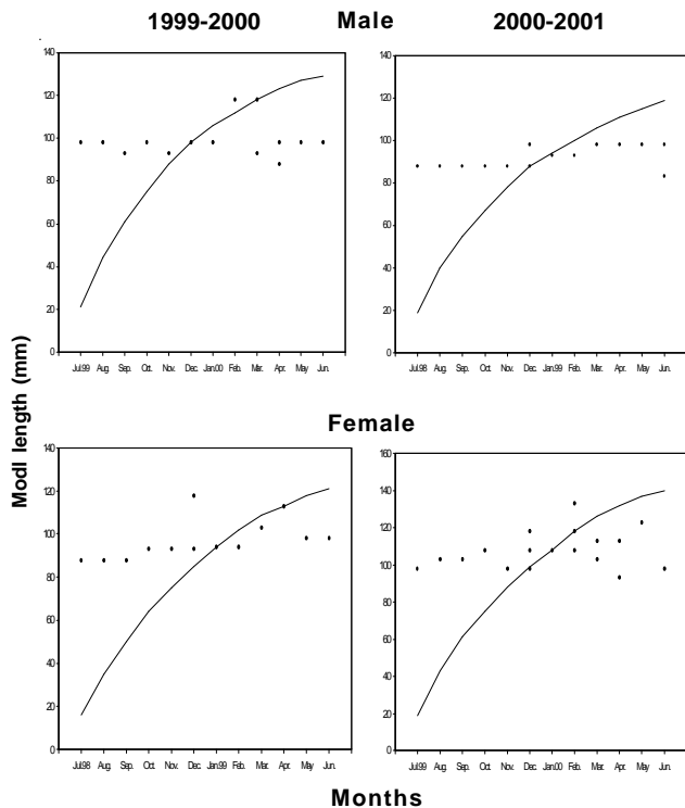
Image 5. Scatter diagram of modal length-month for Salmostoma untrahi
